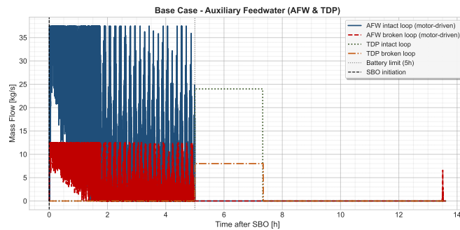
Figure 13: Auxiliary and Turbo-Driven Pump Flow
